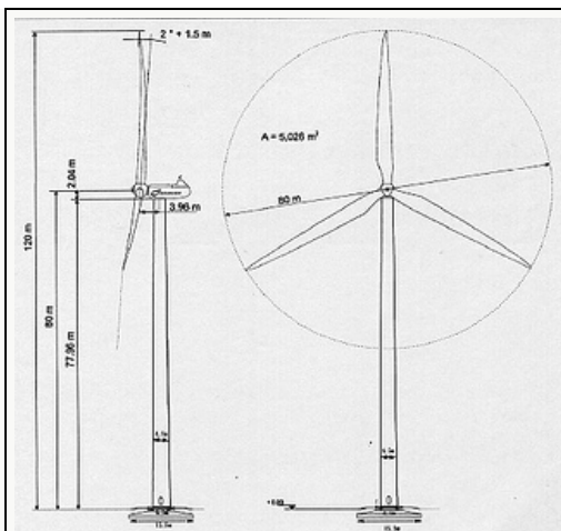
Fan design, the height of a wind turbine, plus blades, up to 120 meters, equivalent to the height of 40 storeys.
